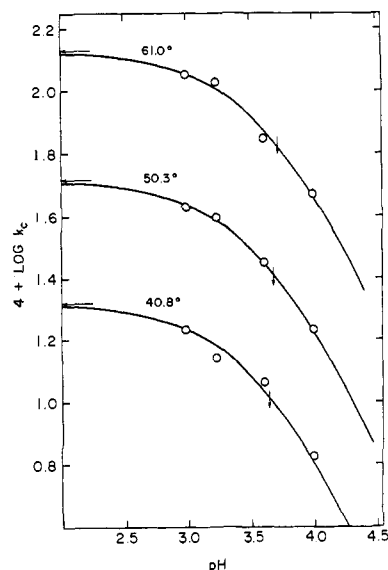
Figure 4. The pH-log rate profile for cycloheptaamylose-catalyzed 3'-chlorobenzoylactic acid decarboxylation. The solid lines were obtained by fit of eq 5 to the experimental points. Horizontal arrows represent the y intercept, \log k_{c1} , and vertical arrows are pK_{cA} values.
