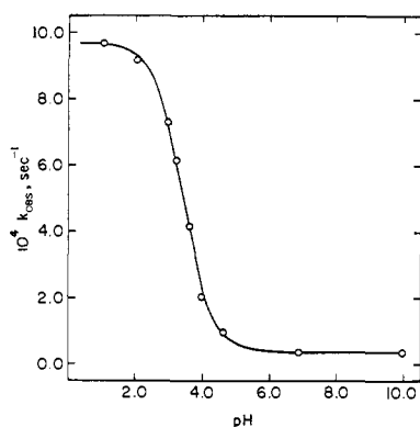
Figure 1. The pH-rate profile for aqueous 4'-methylbenzoylactic acid decarboxylation at 50.3°. The solid line was drawn using constants from Table I and the expression for k_{obsd} derived from eq 2.
