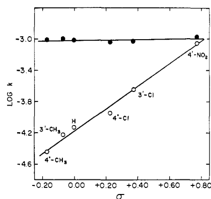
Figure 2. Hammett plot for aqueous benzoylactic acid (●) and anion (○) decarboxylation at 50.3°. The solid lines have slopes of +0.031 and +1.42 for acid and anion decarboxylation, respectively.
