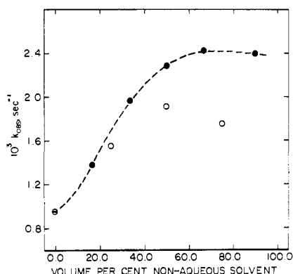
Figure 3. The effect of 2-propanol (●) and acetonitrile (○) on benzoylacetic acid decarboxylation at 50.3^\circ . All solutions were 0.1 M hydrochloric acid.
